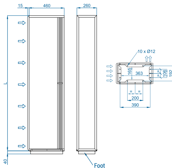
Vertical installation
