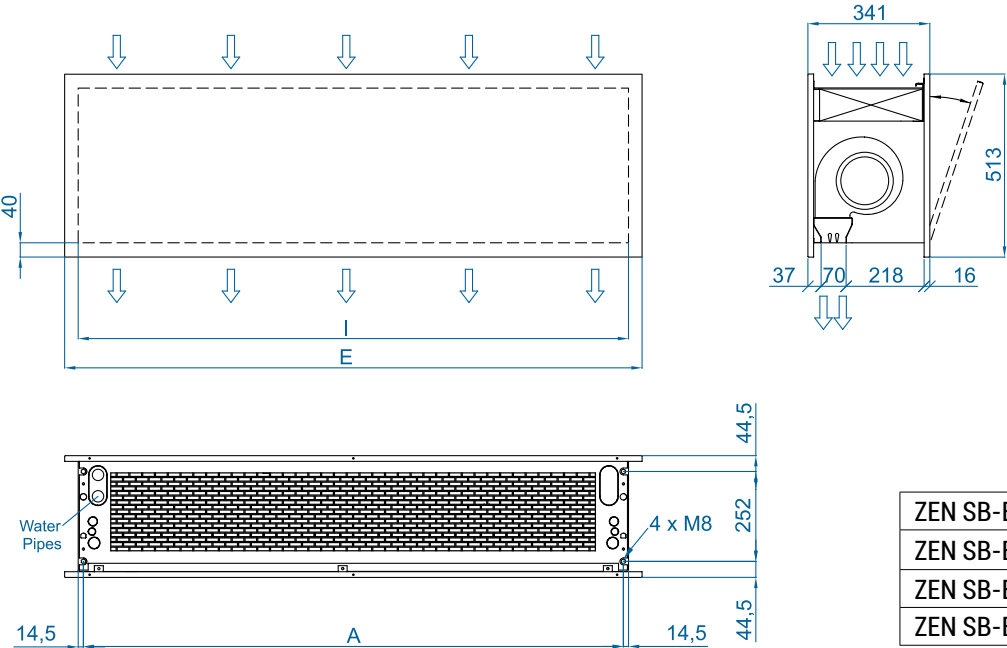
Horizontal installation
